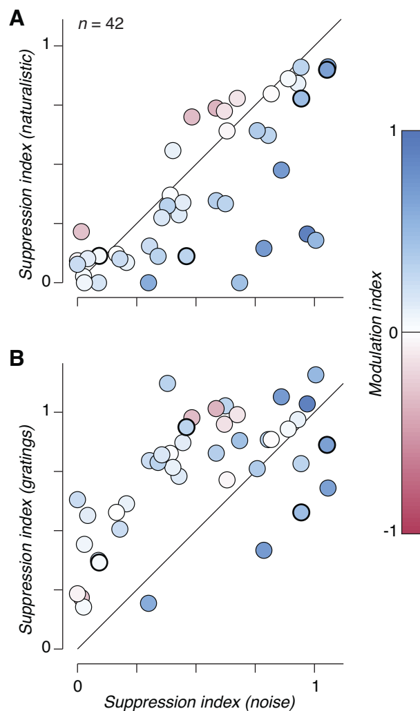
Fig. 5. Surround suppression strength depends on naturalistic statistics. A: surround suppression index (fractional reduction in firing rate to large stimuli, see MATERIALS AND METHODS) measured from responses to spectrally matched noise compared with that measured from responses to naturalistic stimuli. Each circle represents the suppression index for a neuron computed from the average responses to all families tested with size-varying apertures. Circles are colored according to the modulation index measured for the largest size stimulus. Suppression was significantly stronger in response to noise than to naturalistic stimuli ( P < 0.005 , paired t -test). Circles surrounded by a thick black line indicate values averaged across families for the 4 neurons depicted in Fig. 2. B: surround suppression index measured from responses to spectrally matched noise compared with that measured from responses to full-contrast drifting sinusoidal gratings. Circles are colored as in A. Suppression was significantly stronger in response to gratings compared with noise stimuli ( P < 0.001 , paired t -test).
