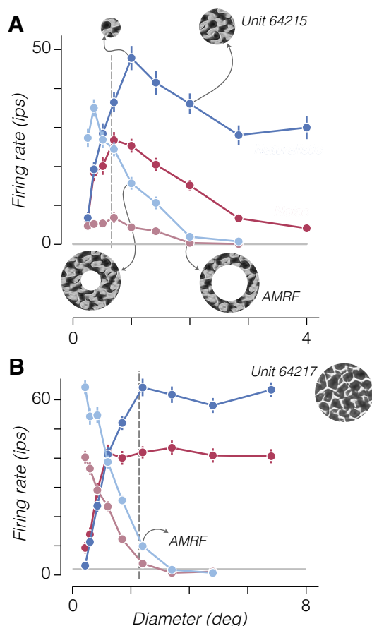
Fig. 8. Responses to annular stimuli reveal surround facilitation to naturalistic stimuli. A: saturated color traces show responses of an example cell to a circular patch of noise (red) or naturalistic (blue) texture. Desaturated color traces show responses to an annular patch. The x-axis indicates the outer diameter of circular patches and inner diameter of annular patches. Inset images show example circular ( top ) and annular ( bottom ) stimuli with matched outer and inner diameters, respectively. The example annular stimulus at bottom right represents the size of the annular minimum response field (AMRF) for the neuron, because naturalistic stimuli windowed within an annulus with this inner diameter drove a response above the spontaneous rate. Error bars represent \pm SE across samples and repetitions. Gray horizontal line represents mean spontaneous activity. Dashed vertical line represents the classical receptive field size estimate from gratings. B: responses from a different example cell exhibiting no surround suppression and a strong preference for naturalistic over noise stimuli presented within an annulus for all sizes that drive a response. Inset image shows an example of the texture family used to stimulate the neuron. Arrow indicates diameter of the AMRF for this neuron; ips, impulses/s.
