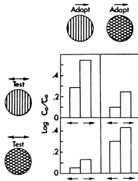
Fig.7. The effects of adaptation to moving gratings and plaids on the detectability of gratings and plaids. Contrast threshold elevation is the ratio of adapted to unadapted contrast threshold, expressed in log units. The two bars of each histogram represent the effects on test stimuli moving in the adapted and unadapted direction, as indicated by the arrows. The data shown are the means of values obtained for three observers; the standard error of the mean was about 0.025 log units.
