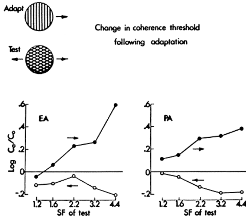
Fig. 8. The effect of grating adaptation on the coherence threshold for plaids. The adapting grating was constant, and coherence was tested for plaids of several spatial frequencies moving in the adapted (filled symbols) and unadapted directions (open symbols). Threshold elevation is the ratio of adapted and unadapted coherence thresholds, expressed in log units. The standard error of the mean was about 0.05 log units.
