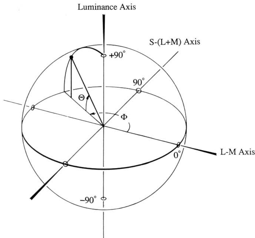
Fig. 1. Color space used to describe the stimuli. The origin is a neutral white. Along the L - M axis, excitation of the L- and M-cones covaries so as to leave their sum constant. Along the S - (L + M) axis only the excitation of the S-cones changes. Along the luminance axis, the excitation of all three cone types is varied in proportion to their excitation at the white point. \Phi denotes the azimuth of a stimulus vector, and \Theta its elevation out of the isoluminance plane.
