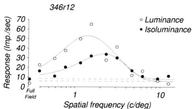
Fig. 7. Example spatial-frequency tuning curve for luminance (open symbols) and isoluminant (filled symbols) gratings. The solid lines show the best fits of a smooth function (difference of exponentials). The dashed lines show the baselines for the two experiments. This cell had a preferred temporal frequency of 3.75 Hz for luminance gratings. It did show a response minimum (with a significant response) at an elevation of -11 deg in the elevation experiment.
