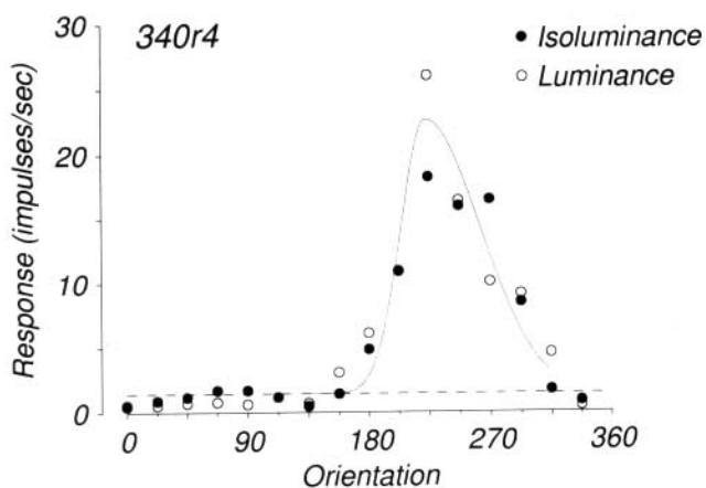
Fig. 10. Example orientation tuning curve for luminance (open symbols) and isoluminant (filled symbols) gratings. The solid curve shows the best fit of a smooth function (asymmetric Gaussian) to the luminance data points. The dashed line indicates the response baseline. This cell showed a response minimum (at about twice the spontaneous firing rate) at an elevation of +2 deg. Its preferred spatial frequency was 1.2 cycles/deg, and its preferred temporal frequency was 7.5 Hz for luminance gratings.
