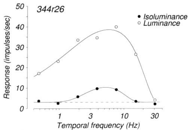
Fig. 9. Example temporal-frequency tuning curve for luminance (open symbols) and isoluminant (filled symbols) gratings. The solid curves show the best fit of a smooth function (difference of exponentials). The dashed line indicates the response baseline. This cell had a preferred spatial frequency of 0.4 cycles/deg for both luminance and isoluminant stimuli. In the elevation experiment it had a complete null at an elevation of 1 deg.
