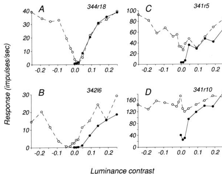
Fig. 4. Typical response patterns observed in the elevation experiment as a function of luminance contrast. The open symbols indicate the response to stimuli having a chromatic component. The closed symbols indicate the responses to purely luminance stimuli. Baseline responses were subtracted. For chromatic stimuli, the contrast of the chromatic component was fixed at 75% of the maximum of our monitor. A: This cell was representative of the most common type. It had a complete null very close to the photometric isoluminant point. The response was fully explained by the luminance component of the stimulus. For this cell the temporal frequency was 7.5 Hz, spatial frequency was 0.4 cycles/deg, and azimuth was 22.5 deg. B: This cell had a null at an elevation close to photometric isoluminance. Its response could also be attributed solely to the luminance component of the stimulus. The preferred temporal frequency for this cell was 7.5 Hz, spatial frequency was 0.4 cycles/deg, and azimuth was 157.5 deg. C: This cell had a minimum response close to isoluminance, but the response did not decrease to baseline. For higher luminance contrasts, the response curves for luminance and color overlapped. Temporal frequency was 7.5 Hz, spatial frequency was 0.4 cycles/deg, and azimuth was 10 deg. D: This cell did not show a minimum response over the range of elevations we used. For this cell the temporal frequency was 3.75 Hz, spatial frequency was 2.3 cycles/deg, and the azimuth was 0 deg. We tested this cell with gratings of different spatial frequencies and the peak spatial frequency for isoluminant gratings was equal to that for luminance.
