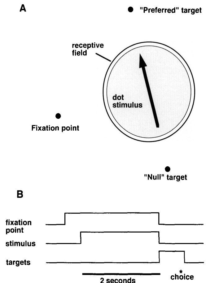
Fig. 1. Schematic of the behavioral task and stimulus configuration used in these experiments. A: Spatial configuration. The outer circle denotes the receptive field of the neuron under study, and the inner shaded region the random dot stimulus. This stimulus can be in either the neuron's preferred direction or its opposite ("null"). Response targets, which were small spots of light from projection LEDs, were aligned with the two possible directions of motion along a diameter of the stimulus. In some circumstances, we would shift these away from collinear alignment to reduce choice biases. B: Timing of events in a trial.
