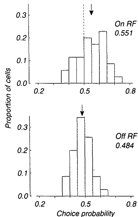
Fig. 9. Dependence of choice probability on the location of the stimulus. The choice probability for each of these 33 cells was measured in two ways: with the visual stimulus either on (upper histogram) or off (lower histogram) the cells’ receptive fields, as described in the text. All other stimulus parameters remained the same.
