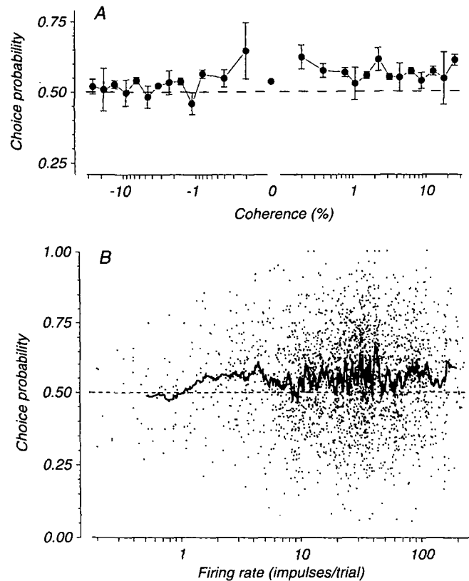
Fig. 3. Dependence of choice probability on stimulus coherence and neuronal response. A: The average relationship between stimulus coherence and choice probability for all 299 cells in our sample. Negative coherence values indicate null direction motion. Each point represents the average choice probability for all cells for which a choice probability could be measured at that coherence level. The error bars represent the standard error of the mean; large errors typically mean that the coherence level was rarely employed in our experiments. B: The relationship between mean neuronal firing rate and choice probability for 2668 stimulus conditions for the 299 cells in our sample. Each point represents the calculated choice probability for a single stimulus. The jagged line shows the running mean of 41 adjacent observations.
