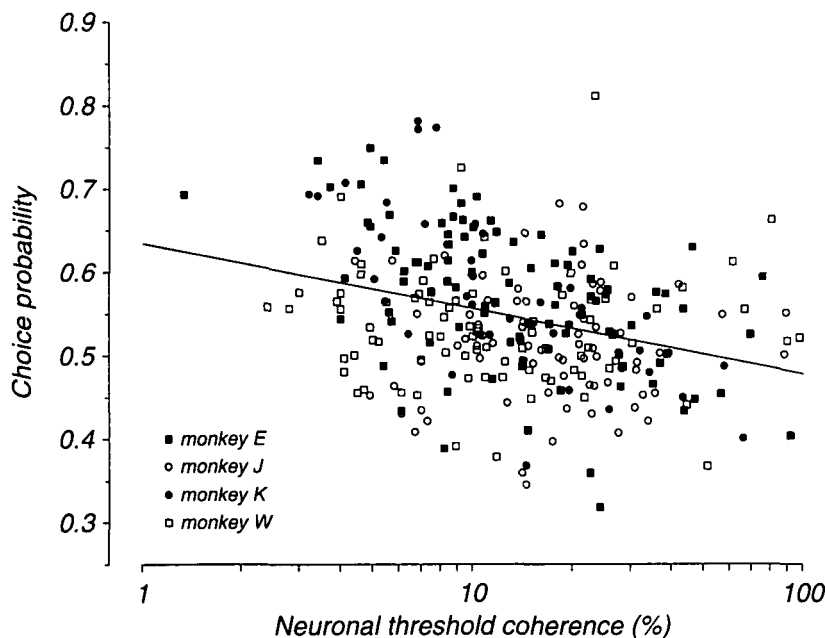
Fig. 13. Relationship between choice probability and neuronal threshold. The neuronal threshold was derived from an analysis presented elsewhere (Britten et al., 1992); it corresponds to the lowest stimulus coherence at which the neuron's response could be used to distinguish preferred from null direction motion on 82% of trials. The relationship portrayed here differed considerably across monkeys; the two animals with the highest average choice probability (E and K) were the only ones to show a significant relationship individually. These two animals' data are drawn with solid symbols. Choice probabilities were derived from all stimulus conditions combined; similar effects were observed when choice probabilities for different directions of motion were compared separately.
