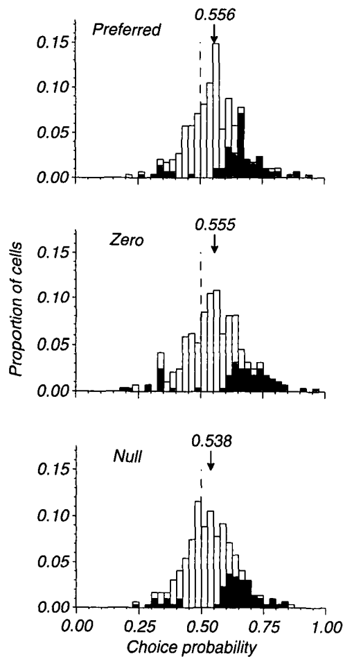
Fig. 5. Distributions of neuronal choice probability for all 299 cells in the sample, compiled separately for preferred direction (296 cases; a few lacked sufficient trials for analysis), null direction (293 cases), and zero coherence (287 cases) responses. Stippled bars indicate cases that were significantly different from 0.5 by the permutation test described in the text.
