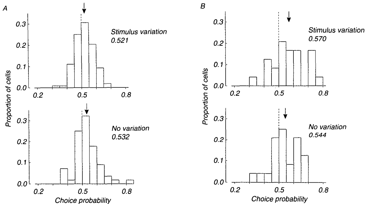
Fig. 8. Dependence of choice probability on the presence of trial-to-trial variance in the stimulus. A: Distributions of choice probability for 108 cells from monkeys W and J studied with stimulus variation (upper histogram) compared with that for 43 different cells from the same monkeys studied with no variation (lower histogram). B: Choice probability distributions for 24 cells from monkey E for which we made interleaved measurements with both types of stimulus. Both measurements were made with 0% coherence stimuli which were randomly interleaved within blocks of trials that also contained stimuli with non-zero coherence.
