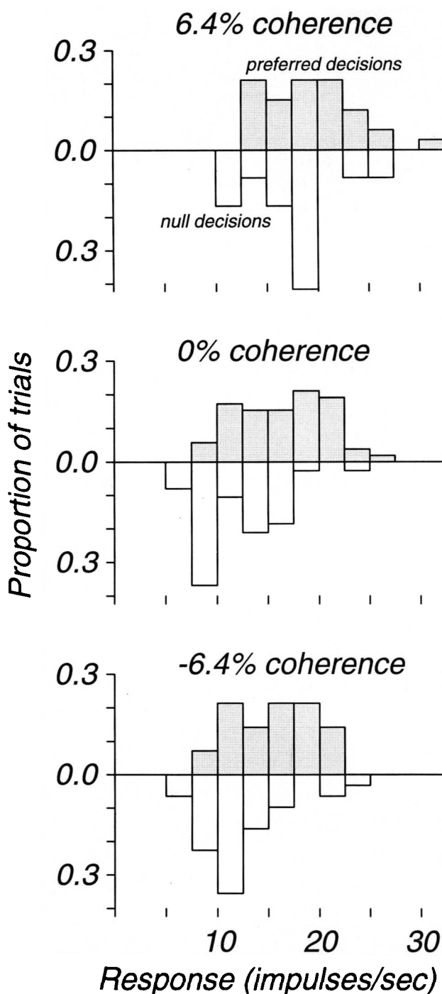
Fig. 2. Response distributions from a representative MT cell which showed a substantial trial-to-trial covariation between firing rate and behavior. Each panel represents a single stimulus coherence and direction; the -6.4\% condition corresponds to null direction motion. The upper histograms (stippled) show firing rates on trials on which the monkey decided in favor of the preferred direction, and the lower histograms (open) show the firing rates on trials on which the monkey made the opposite decision.
