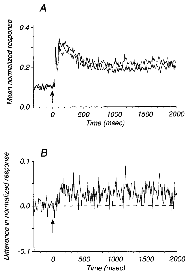
Fig. 11. Time course of the firing rate difference that underlies the choice probabilities. The 0% coherence responses of 75 cells that showed a significant choice probability were combined. Each cell gave a pair of averaged response histograms (bin width: 10 ms) corresponding to preferred and null direction decision trials. Each pair was normalized to the peak of the preferred direction histogram. A: Pooled average response histograms for each response direction, with the upper representing the preferred direction decision trials and the lower showing the null direction decision trials. B: The difference between the two responses as a function of time. Note that the response difference is only present during the visual stimulus period, and not during the fixation period prior to stimulus onset (arrows).
