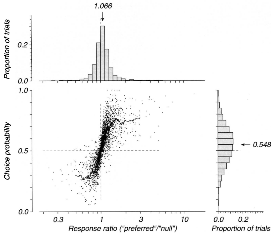
Fig. 4. The relationship between choice probability and firing rate ratios between preferred and null choice trials, for the same set of observations shown in Fig. 3B. The marginal distributions show the distribution of each measure, and the arrows indicate the corresponding means. The jagged line is a running mean of 41 adjacent observations.
