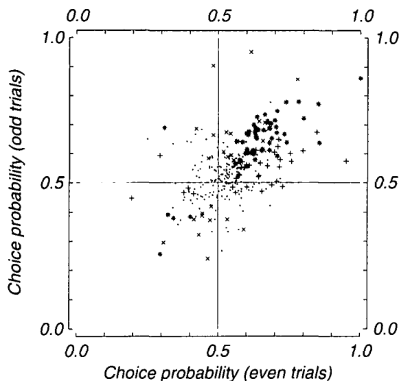
Fig. 7. Comparison of choice probability calculated from the odd and even trial subsets used in Fig. 6. Values that differed significantly from chance by the permutation test on the even subset are shown by +, on the odd subset by x, on both subsets by *, and on neither by a point.
