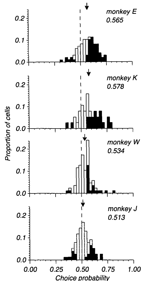
Fig. 12. Choice probability distributions from the four monkeys (monkey E: 97 cells; monkey K: 38 cells; monkey W: 87 cells; and monkey J: 77 cells). The choice probabilities were pooled for all stimulus conditions. The stippled bars, as in Fig. 5, indicate neurons whose choice probabilities differed significantly from 0.5 on the permutation test.
