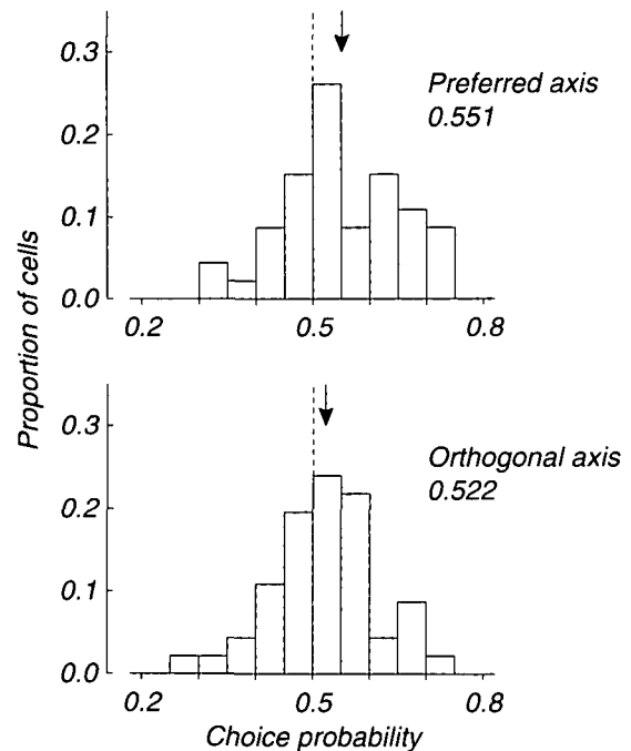
Fig. 10. Dependence of choice probability on the axis of motion of the stimulus. The choice probability for each of these 45 cells was measured in two ways: with the visual stimulus moving along the neuron's preferred axis (upper histogram), or roughly orthogonal to it (lower histogram).
