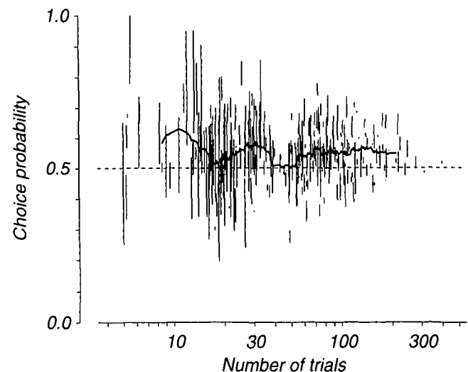
Fig. 6. Repeated-measure reliability of the choice probability for 294 of the 299 neurons (five neurons were omitted because of an insufficient number of trials). Each vertical line connects two values of the estimated choice probability for each neuron, calculated separately for even and odd numbered trials. The solid line through the center of the graph plots the running average of 21 adjacent observations, ordered by number of trials. Four types of trial are used for each calculation (preferred and null direction decisions for each subset of trials), and the values on the abscissa correspond to the average number of entries for these trial types.
