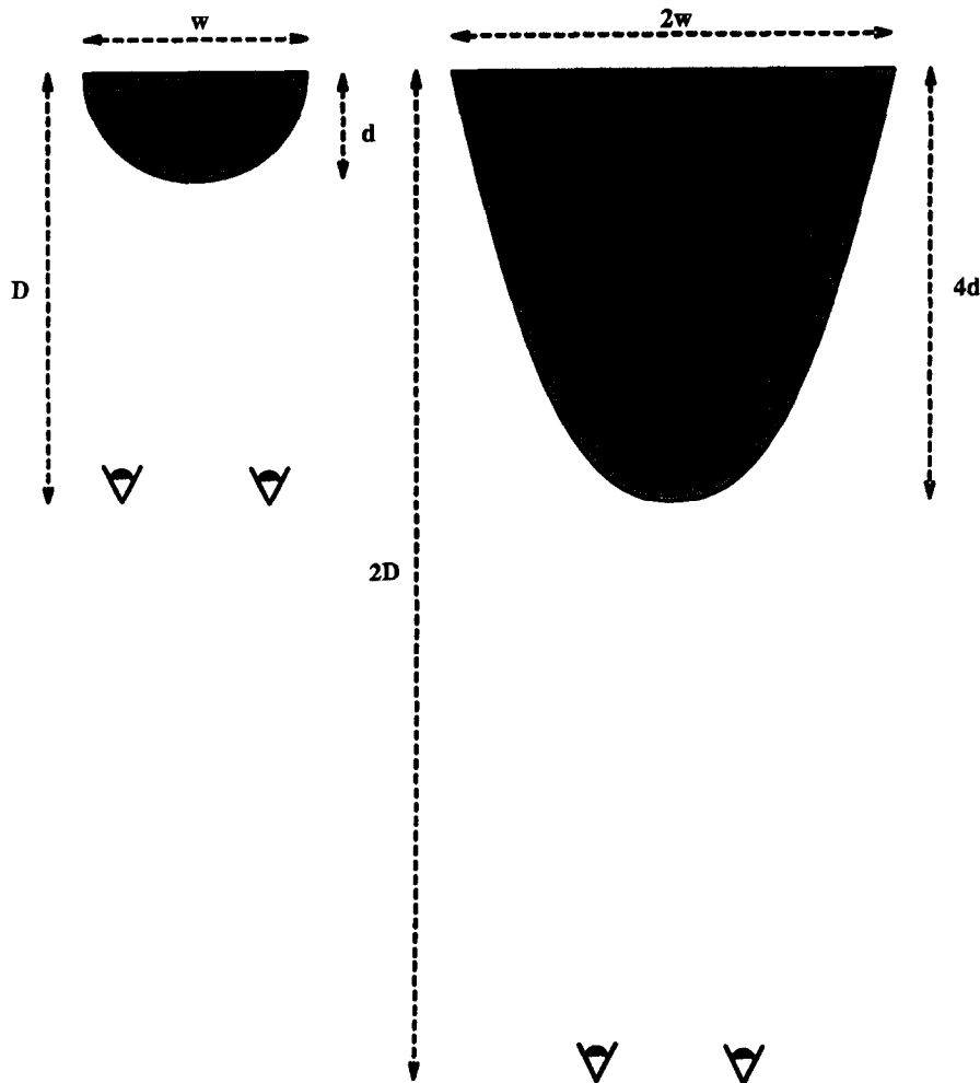
FIGURE 1. Stereo scaling problem. The filled arcs illustrate cross-sections through the cylinders depicted by the same disparity field viewed from two distances. When the viewing distance ( D ) is doubled for the same disparity field the depths depicted by those disparities are quadrupled. The width calculated from the visual angle subtended by the fronto-parallel extent of the shape is only doubled. Thus, there is a change in the depth/width ratio of the cylinder when the viewing distance used to scale the disparity field is changed.
