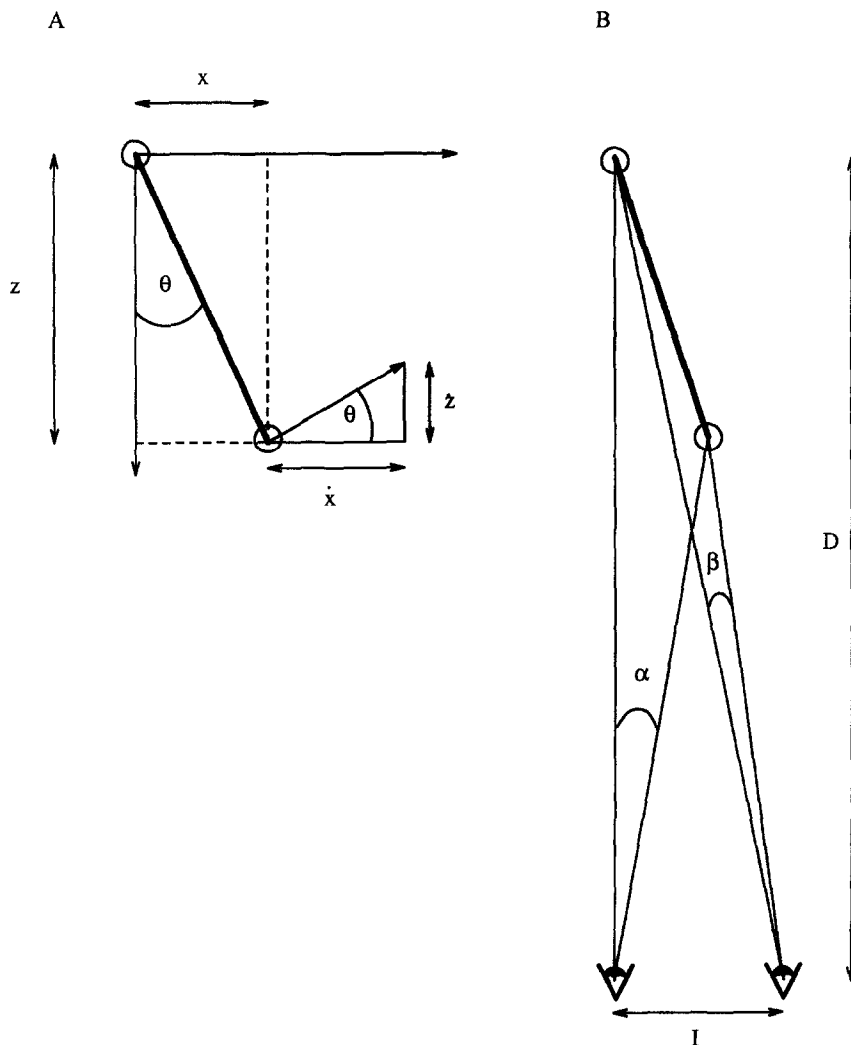
FIGURE A1. Schematic diagram of a stereo-motion integration scheme. (A) The heavy line joins two points in relative motion. The origin is coincident with the left point. The two angles \theta are equal, but the sides of the triangles are measured by different visual parameters. This allows the viewing distance D , to be eliminated from equations for z and x (see text). (B) The disparity \eta is the difference in visual angle subtended by the two points, \alpha - \beta . D marks the viewing distance and I the interocular separation.
