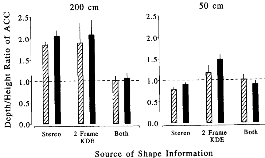
FIGURE 7. The depth/height ratio for the apparently circular cylinder data plotted for three conditions. Increased depth/height ratio indicates decreased perceived depth. Condition 1: stereo alone replotted from Fig. 5. Condition 2: two frame KDE, monocularly viewed. Condition 3: two frame KDE plus stereo, four frames in total, two to each eye. Hatched bars, subject EBJ; solid bars, subject RBC. Data for viewing distances of 200 and 50 cm are shown.
