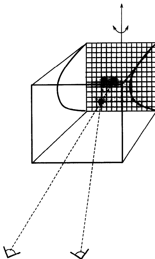
FIGURE 2. The geometry used in stimulus generation. The emboldened arcs indicate the occluding contours of a cylindrical surface. The surface is embedded in a volume filled with texture elements. The back plane of the volume is the image plane, where the pixel array is indicated by hatching. To generate each eye's image a line is traced from that eye's view through the surface to an image pixel (shown as a dashed line). That pixel is set to the colour of the surface at the point of intersection (marked with a solid circle). This process is repeated for each image pixel. The disparity between the two eyes' views can be seen from the separation of the two marked pixels on the image plane. The vertical axis of surface rotation is marked.
