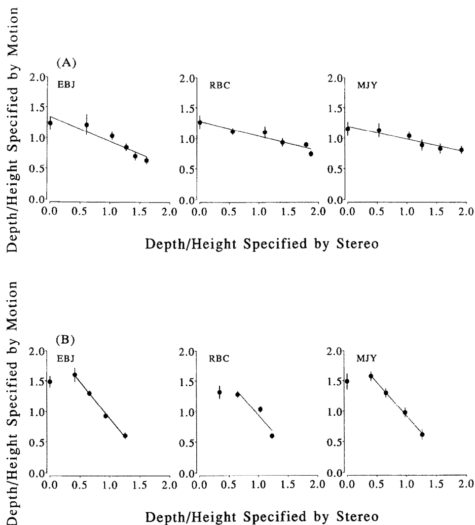
FIGURE 6. Apparently circular cylinder data for surfaces with incongruent depths specified by kinetic depth and stereo. The data are plotted in terms of the depth/height portrayed by stereo and the depth/height portrayed by motion for the cylinders which were judged to have equal apparent depth and height. In terms of the abbreviations used in the text the ordinate is d_m/h , and the abscissa is d_s/h . Each data point corresponds to a different portrayed d_s/d_m ratio. The error bars show standard deviations. (A) Viewing distance 200 cm. The lines shown are regression lines. The goodness of fit of the regression lines can be estimated from the closeness of the squared correlation coefficient to 1. The r^2 values are EBJ, 0.872; RBC, 0.892; MJY, 0.891. (B) Viewing distance 50 cm. The lines shown are regression lines fit to all points but the leftmost, thus taking account of only the linear portion of the data set (see text). The r^2 values are EBJ, 0.996; RBC, 0.892; MJY, 0.997.
