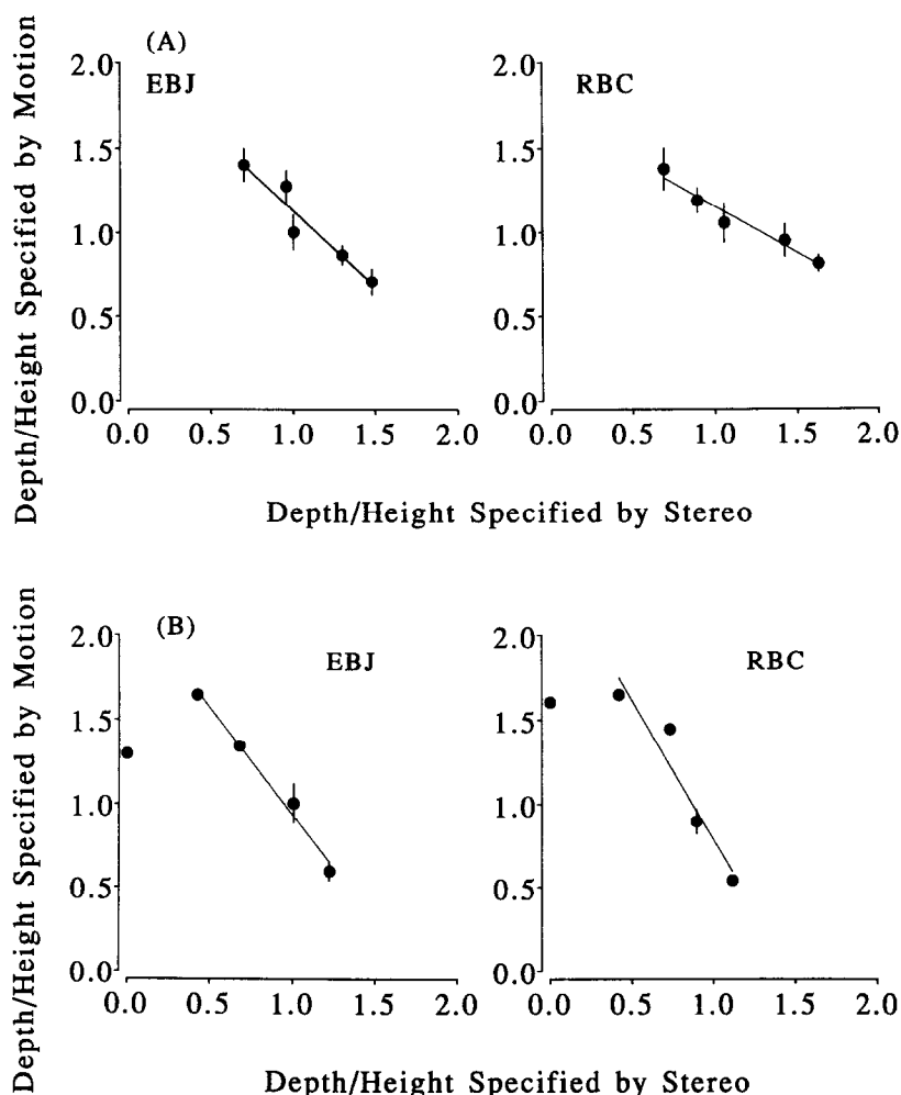
FIGURE 8. Incongruent combinations of stereo and motion, with two frame motion. The data are plotted in terms of the depth/height portrayed by stereo and the depth/height portrayed by motion for the cylinders which were judged to have equal apparent depth and height. (A) 200 cm viewing distance. The r^2 values are EBJ, 0.907; RBC, 0.956. (B) 50 cm viewing distance. The lines shown are regression line fits to the data (excluding the 0 point for the 50 cm data). The r^2 values are EBJ, 0.982; RBC, 0.926. The error bars show standard deviations. Comparison with Fig. 6 shows that stereo has a greater effect when the motion cue is weakened (the absolute slopes of the regression lines are larger here than in Fig. 6).
