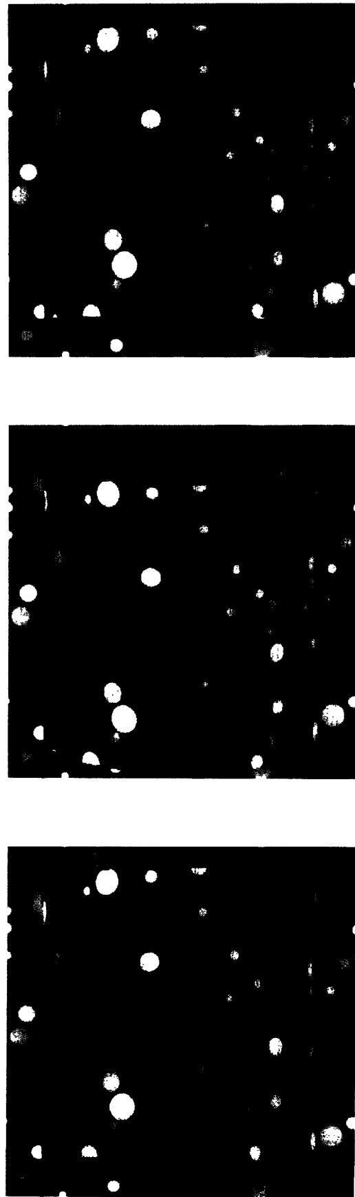
FIGURE 3. Example stimulus. A stereo pair which formed one frame of a motion stimulus. The images were traced for a circular cylinder to be displayed at 50 cm, rotated 3 deg anti-clockwise. The images are not exactly to scale, thus the disparity field is not as it would be in the experiments.
