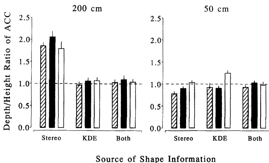
FIGURE 5. Portrayed depth/height for cylinders which appeared circular to the three subjects. Height actually refers to half-height of the cylinder which was fixed at 3 cm. The data are plotted in terms of depth/height yielding an inverse scale—larger values represent decreased perceived depth. The dashed line indicates veridical perception where portrayed height equals depth. Hatched bars, subject EBJ; solid bars, subject RBC; open bars, subject MJY. Data for viewing distances of 200 and 50 cm are shown.
