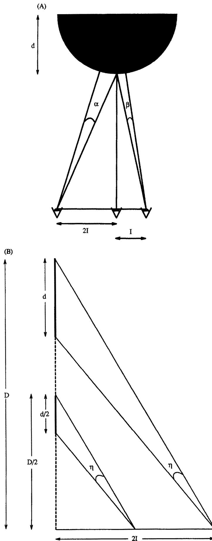
FIGURE 4. How stereo and motion depths are independently manipulated. The interocular separation parameter used in ray-tracing is varied. (A) The consequence of doubling the interocular separation ( I ) is that disparity generated by the depth ( d ) is doubled— \alpha is twice the size of \beta . Manipulating the interocular separation to change the depth specified by disparity does not alter the depth depicted by each eye's flow field. (B) The disparity ( \eta ) generated by doubling the interocular distance is exactly equivalent to that generated by an object of half the size at half the distance (proven here by similar triangles). Changing the interocular separation is equivalent to changing the viewing distance in terms of the size of disparity generated.
