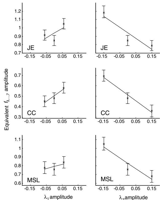
Fig. 5. Experimental results. Left-hand column: A_{\rho_1^-} , A_\rho and A_{\rho_1^+} are plotted against the values -\varepsilon_1 , 0, and \varepsilon_1 . That is, for each value of \lambda_1 amplitude, we plot the amount of f_{3,\dots,7} alone that would have resulted in equivalent performance. If the Minkowski exponent is 1 or \infty , the slope of the best-fitting straight line through these three points provides an estimate of 2f_B \cdot \lambda_1 . Right-hand column: analogous results for \lambda_2 .
