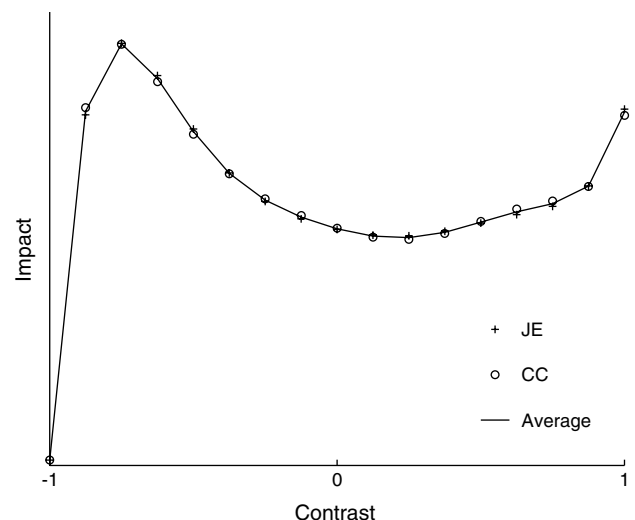
Fig. 3. The discriminator f_{3,\dots,7} . This function was found by Chubb et al. (1994) to govern discrimination within the modulator space A_{3,\dots,7} . Specifically, for all modulators m \in A_{3,\dots,7} , the probability of discriminating m was found to be a function of |f_{3,\dots,7} \cdot m| .
