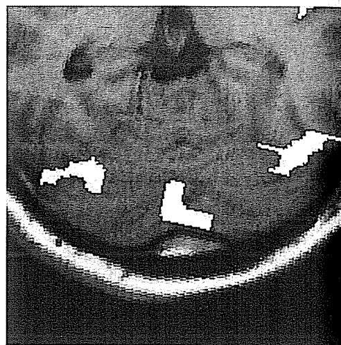
Figure 3-14. Activity of the cerebellum during a saccadic task as revealed by functional magnetic resonance imaging (fMRI). The subject was making voluntary, self-paced saccades between two visible targets. There is increased metabolic activity in the midline cerebellum (dorsal vermis and underlying fastigial nuclei) and also in the cerebellar hemispheres. Similar activation occurred if saccades were made in darkness between remembered target locations. (Courtesy Dr. Manabu Honda of Kyoto, Japan.) (From Honda M, Zee DS, Hallett M. Cerebellar control of voluntary saccadic eye movements in humans. Soc Neurosci Abstr 15, 1189, 1997.)
