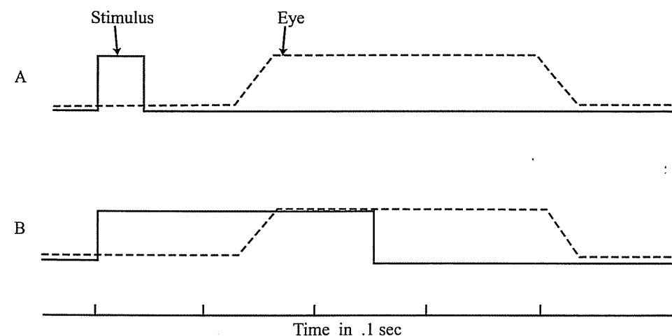
Figure 3–7. Saccadic eye movement responses to double-step target jumps. Horizontal position is on the ordinate scale. Note that the intersaccadic interval remains constant in spite of the different durations (compare A and B) between the two target jumps. (Reproduced, with permission, from Westheimer G. Eye movement responses to a horizontally moving visual stimulus. Arch Ophthalmol 52, 932–941, 1954. Copyright 1954, American Medical Association.)
