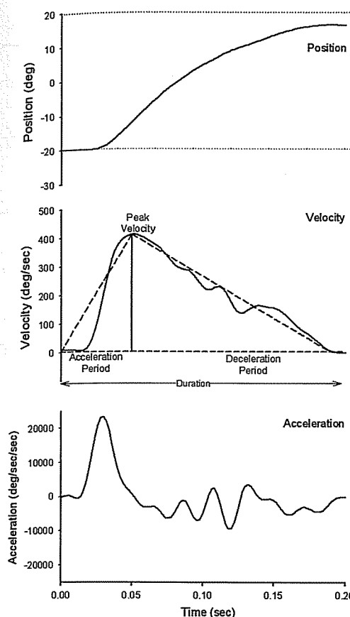
Figure 3-1. Representative record of a 36-degree horizontal saccade made by a normal subject in response to a 40-degree target jump (dotted lines in top panel). Corresponding position, velocity, and acceleration records for this saccade are shown. In the middle panel, components of the velocity waveform are shown, including the acceleration period and total duration, the ratio of which gives a measure of the skewing of the velocity waveform. Positive values correspond to rightward movements.
