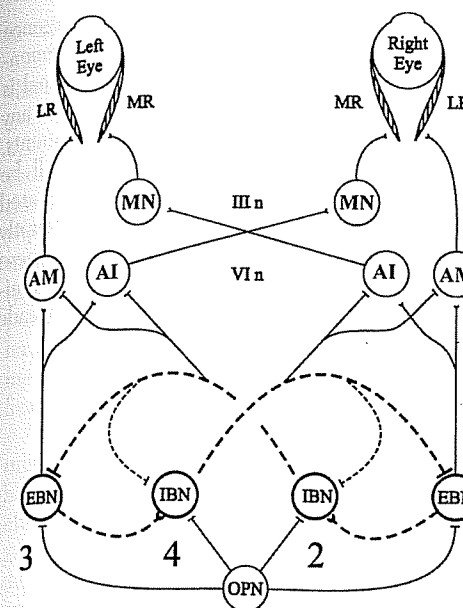
Figure 3-10. A brainstem neural network model for generation of horizontal saccades. Projections with flat ending are inhibitory, the others excitatory. Saccades require reciprocal innervation to the medial rectus (MR) and lateral rectus (LR) of both eyes. The LR is driven by the ipsilateral abducens nucleus (VI n) motoneurons (AM). The VI n also contains abducens internuclear neurons (AI) that send their axons to the contralateral oculomotor nucleus (III n), which drive the MR of the other eye. Excitatory burst neurons (EBN) provide the saccadic drive to ipsilateral AM and AI. EBN also project to inhibitory burst neurons (IBN). IBN provide inhibition to the contralateral AM and AI. Thus, an EBN/IBN pair provides reciprocal innervation. IBN also provide inhibition to the contralateral EBN and IBN. A consequence of this cross-coupling is that the EBN/IBN pairs form a short-latency, positive feedback loop. When omnipause neurons (OPN) are active, they prevent this loop from oscillating. At the beginning of a saccade, OPN neurons cease discharge allowing one set of EBN (1) to start firing and activate ipsilateral IBN (2). During EBN (2) firing, contralateral EBN (3) receive a hyperpolarizing input that keeps them silent. At the end of the saccade, when the IBN (2) cease firing, the EBN (3) start to discharge because of rebound depolarization, which stimulates ipsilateral IBN (4), which, in turn, inhibit the original EBN (1) that fired. Thus, the EBN-IBN pairs tend to spontaneously oscillate whenever the omnipause neurons are inhibited and there is no specified saccadic command. (Adapted from Ramat S, Leigh RJ, Zee DS, Opticon LM. Ocular oscillations generated by coupling of brainstem excitatory and inhibitory saccadic burst neurons. Exp Brain Res 160, 89-106, 2005, with kind permission of Springer Science and Business Media.)
