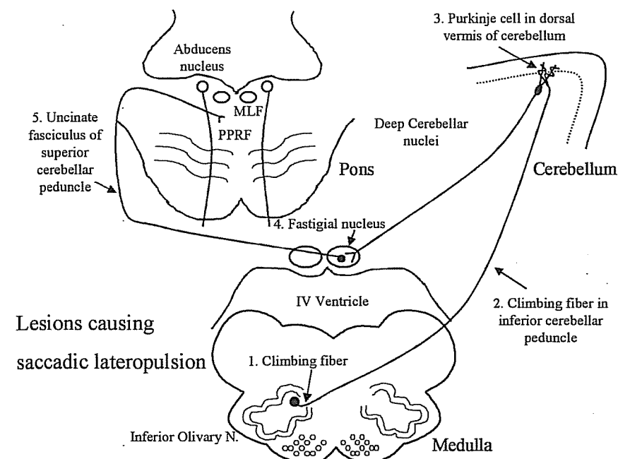
Figure 3-16. Hypothetical scheme to account for lateropulsion of saccades. 584,711,740 Interruption of climbing fibers originating from the inferior olivary nucleus may occur prior to their crossing in the medulla (1) or as they enter the inferior cerebellar peduncle (in Wallenberg's syndrome, (2)). Loss of climbing fiber inputs to Purkinje cells in the dorsal vermis causes the latter to inhibit the fastigial nucleus (4), which causes ipsipulsion of saccades. Pharmacological inactivation of the dorsal vermis (3) causes contrapulsion (although clinical lesions produce bilateral hypometria). Interruption of crossed fastigial nucleus outputs in the superior cerebellar peduncle (uncinate fasciculus, 5) causes contrapulsion. Thus, contrapulsion arises at sites 1, 3 and 5, and ipsipulsion at sites 2-4.
