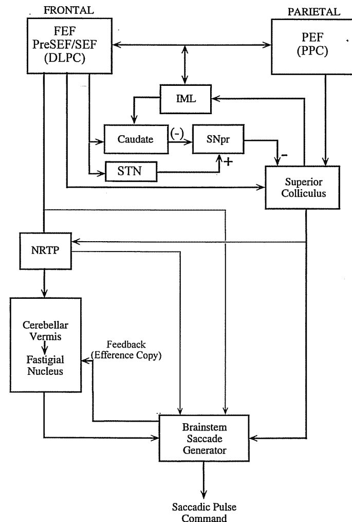
Figure 3-12. Block diagram of the major structures that project to the brainstem saccade generator (premotor burst neurons in PPRF and riMLF). Also shown are projections from cortical eye fields to superior colliculus. DLPC, dorsolateral prefrontal cortex; FEF, frontal eye fields; IML, intramedullary lamina of thalamus; NRTP, nucleus reticularis tegmenti pontis; PEF, parietal eye fields; PPC, posterior parietal cortex; SEF, supplementary eye fields; SNpr, substantia nigra, pars reticulata; STN, subthalamic nucleus. Not shown are the pulvinar, which has connections with the superior colliculus and both the frontal and parietal lobes, projections from the caudate nucleus to the subthalamic nucleus via globus pallidus, and the pathway that conveys efference copy from brainstem and cerebellum, via thalamus, to cerebral cortex. —, inhibition, +, excitation.
