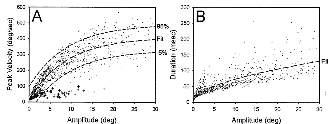
Figure 3-3. Dynamic properties of saccades. (A) Plot of peak velocity versus amplitude of vertical saccades. Data points (dots) are saccades from 10 normal subjects. These normal data are fit with an exponential equation of the form \text{Peak Velocity} = V_{\max} \times (1 - e^{-\text{Amplitude}/C}) , where V_{\max} is the asymptotic peak velocity, and C is a constant defining the exponential rise is shown. Also plotted are the 5% and 95% prediction intervals. The crossed points indicate vertical saccades from a patient with Niemann-Pick type C disease (see Fig. 5B), which lie outside the prediction intervals for normals. (B) Plot of duration versus amplitude. The data from 10 normal subjects are fit with a power equation of the form: \text{Duration} = D_1 \times \text{Amplitude}^n , where D_1 is the duration of a 1 degree saccade, and n is the parameter to be determined.
