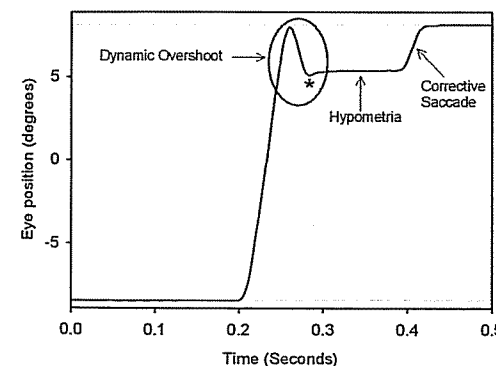
Figure 3-4. Example of a large "dynamic overshoot" in a patient recovering from brainstem encephalitis causing ocular flutter. A small oppositely directed dynamic overshoot (indicated by an asterisk) also occurs. The patient is making horizontal saccades between a stationary target (gray lines). Note that after the initial movement is over, the eye is not on target (it is hypometric) and a subsequent corrective saccade is made. Positive values correspond to rightward movements.
