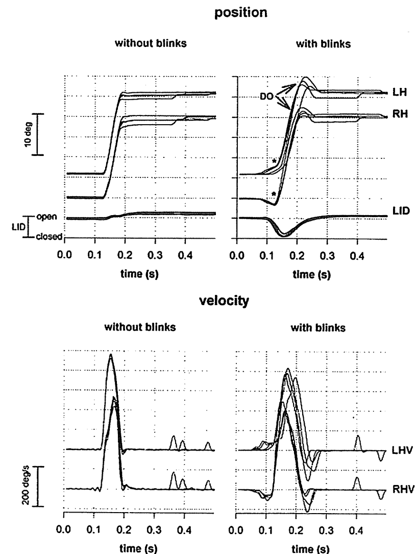
Figure 3-18. Effect of blinks on saccades from a normal subject. Position records are shown above and corresponding velocity traces below. Note that peak velocities are smaller, for similar-sized saccades, when the subject blinks with the saccade. Also note that dynamic overshoots (DO)—oppositely directed postsaccadic movements—occur more frequently with blinks. LH, left horizontal position; LHV, left horizontal velocity; RH, right horizontal position; RHV, right horizontal velocity. (Courtesy of Klaus G. Rottach.)
