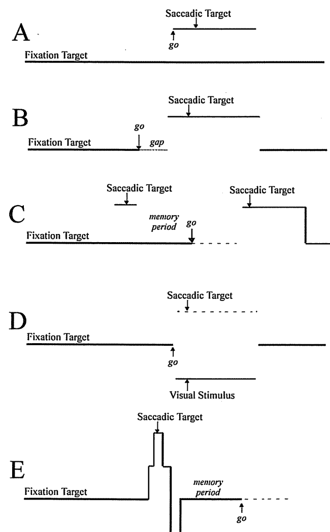
Figure 3-2. Schematic of laboratory stimulus paradigms commonly used to test saccades. In each case "go" indicates the signal for the subject to look toward the "saccadic target." (A) Overlap paradigm, in which the central fixation target stays on throughout. (B) Gap paradigm, in which fixation target is switched off before visual target is switched on. (C) Memory target task. The subject views the fixation target during the time that the visual target is flashed and after several seconds (the memory period), the fixation light is switched off and the subject looks towards the remembered location of the target. (D) The antisaccade task. The subject is required to look in the opposite direction when the visual stimulus is presented. (E) Sequence of saccades task. A series of targets at several locations are turned on in turn. After a memory period, the fixation light goes out as a signal for the subject to make a series of saccades towards the remembered series of target locations.
