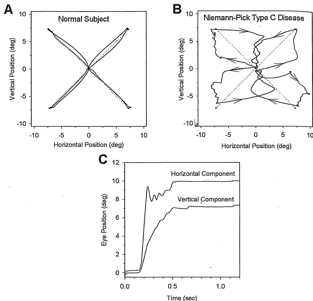
Figure 3-5. Trajectories of oblique saccades. (A) Comparison of trajectories of oblique saccades made to and from four target positions starting at primary position in a normal subject and (B) in a patient with Niemann-Pick type C disease, 599 who showed a selective slowing of vertical saccades. Arrowheads in (B) indicate the direction of eye movement. The trajectory of the target jump is shown as a dotted line. The trajectories of the patient's saccades are strongly curved, reflecting the initial, faster, horizontal component and the later, slower, vertical component. (C) Time plot comparing horizontal and vertical components of an oblique saccade made by the patient with Niemann-Pick type C disease. Horizontal oscillations occurred after the horizontal component had ended, but while the vertical component was still going on. Amplitude-peak velocity plots of vertical saccades made by this patient are shown in Fig. 3-3A.
