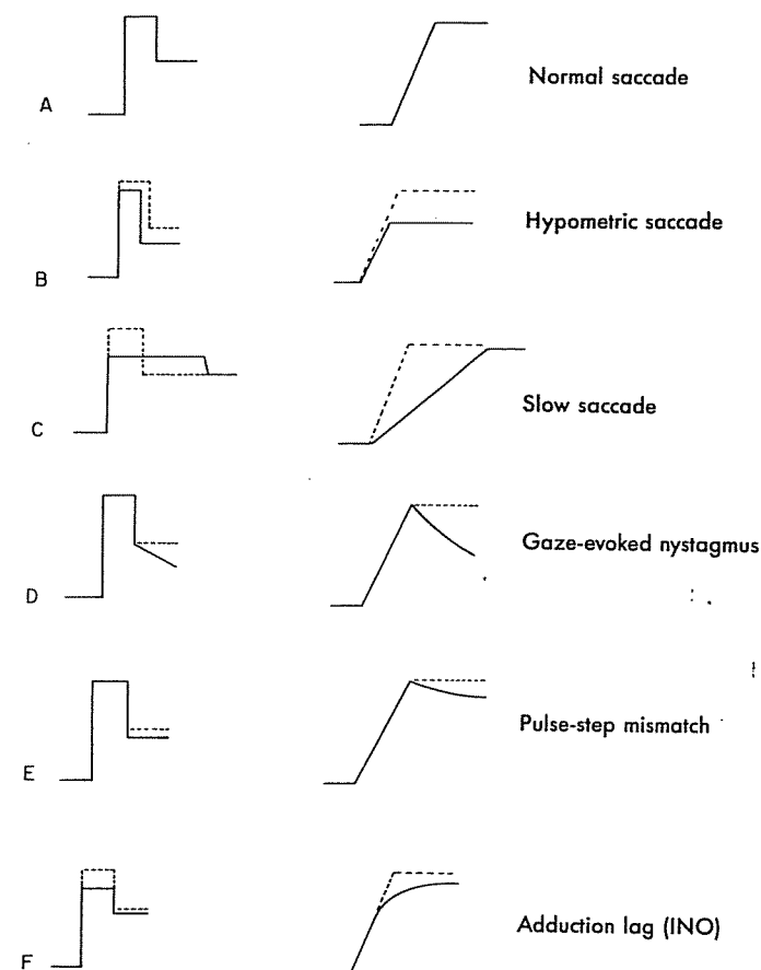
Figure 3-19. Disorders of the saccadic pulse and step. Innervation patterns are shown on the left, eye movements on the right. Dashed lines indicate the normal response. (A) Normal saccade. (B) Hypometric saccade: pulse amplitude (width \times height) is too small but pulse and step are matched appropriately. (C) Slow saccade: decreased pulse height with normal pulse amplitude and normal pulse-step match. (D) Gaze-evoked nystagmus: normal pulse, poorly sustained step. (E) Pulse-step mismatch (glissade): step is relatively smaller than pulse. (F) Pulse-step mismatch due to internuclear ophthalmoplegia (INO): the step is larger than the pulse, and so the eye drifts onward after the initial rapid movement.
