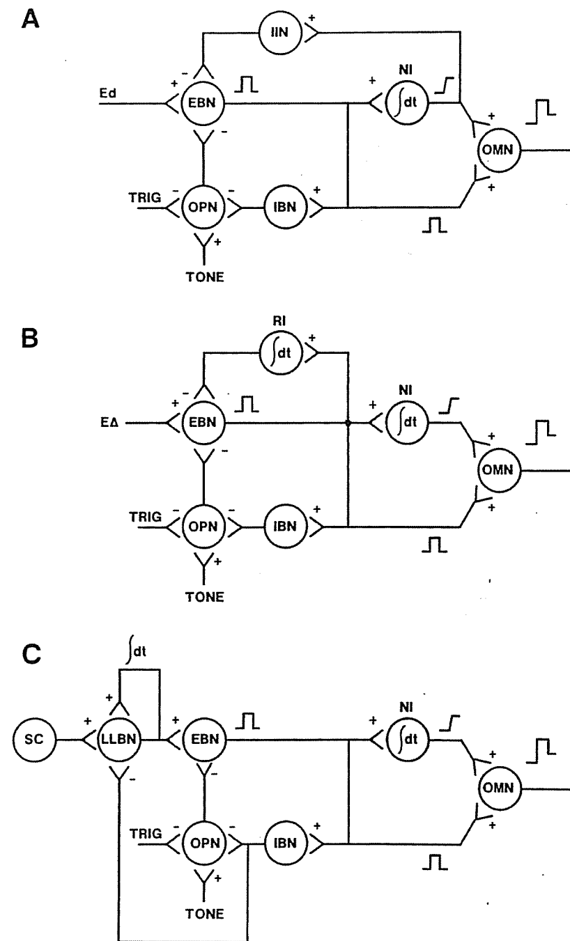
Figure 3-17. Models of the saccadic pulse generator. (A) Model after Robinson. 572 A desired eye position signal (Ed) excites burst neurons (EBN), which in turn project to the ocular motoneurons (OMN), to the neural integrator (NI) and to the inhibitory burst neurons (IBN). Omnipause neurons (OPN) have a tonic level of discharge (TONE) but are inhibited by a trigger signal (TRIG) when a saccade is desired. During the saccade, OPN are kept silent by IBN. The output of the NI is fed back as an efference copy of eye position to EBN via an inhibitory interneuron (IIN). When this signal becomes equal to Ed, the burst neurons cease discharging and the saccade is over. (B) Model after Jürgens and colleagues. 336 The input to the burst neurons is now a desired change in eye position (EA). This signal is compared with an efference copy of eye position, which is now derived from a separate, resettable neural integrator (RI) specific to the saccadic system. (C) Model modified from Scudder. 622 Long-lead burst neurons (LLBN) receive excitatory signals from the superior colliculus (SC) and are the site for the saccade-specific integration of velocity to position signals. The saccade is terminated by comparing the integral of an efference copy of saccade velocity (via IBN) and the integral of the input from the superior colliculus.
