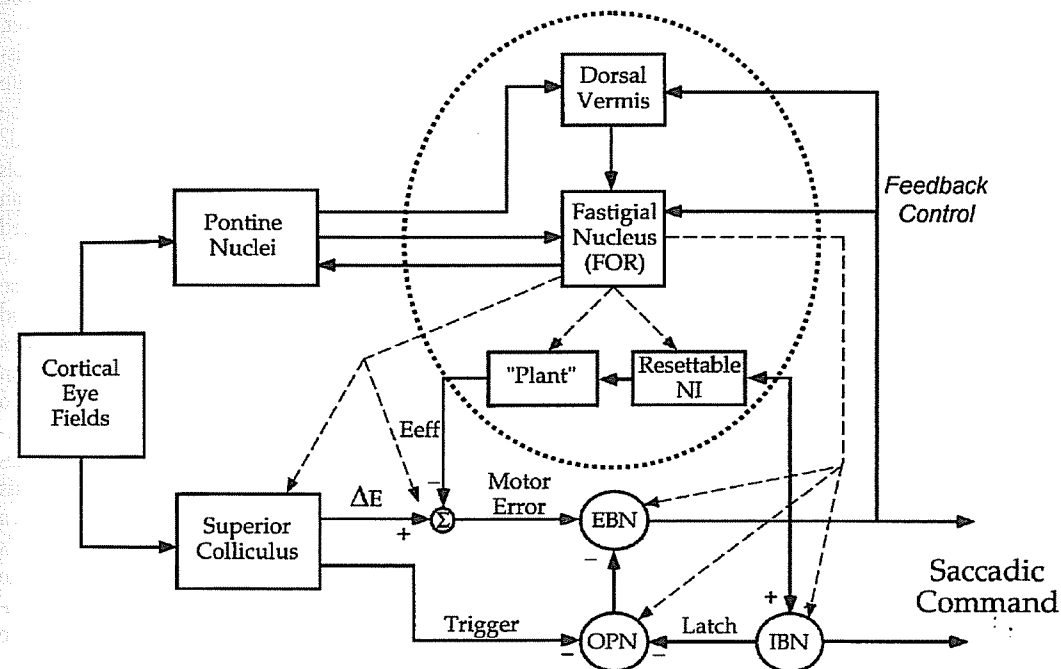
Figure 3-15. Hypothetical scheme for the role of the cerebellum in the generation of saccades. The superior colliculus, and probably the frontal eye field, provide a neural signal representing desired change in eye position ( \Delta E ), which is compared with an efference copy of current eye position ( E_{eff} ), to give motor error, the signal that drives the premotor burst neurons (EBN). The superior colliculus rostral pole also provides the trigger signal to initiate the saccade, which inhibits omnipause neurons (OPN), which then stop inhibiting EBN, and (projection not shown) inhibitory burst neurons (IBN). The EBN project to IBN, which act as a latch circuit to stop OPN from discharging until the end of the saccade (when motor error is zero). The output of EBN and IBN constitute the saccadic command, which projects to ocular motoneurons. To generate E_{eff} , the output of EBN (and IBN, not shown) must be integrated (Resettable NI) and adjusted to account for non-linearities due to the orbital contents ("Plant"). This local feedback circuit may be partly located in the cerebellum. The dorsal vermis and fastigial oculomotor region (FOR) receive inputs from the pontine nuclei, such as NRTP, and climbing fiber inputs from the inferior olive (not shown). The dorsal vermis inhibits FOR, which projects to several elements of the brainstem saccade generator (broken lines), including EBN, IBN, and OPN. The dorsal vermis and FOR could lie within the internal saccadic feedback loop (dotted ellipsoid). -, inhibition, +, excitation.
