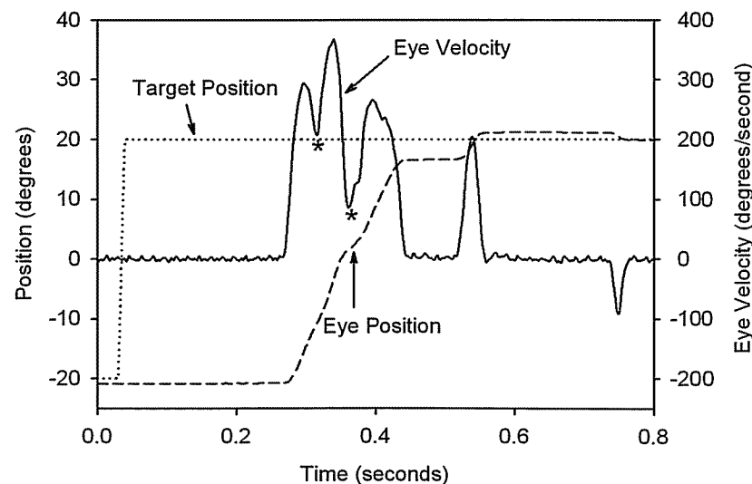
Figure 3-20. Representative records of horizontal saccades made by a patient with late-onset Tay-Sachs disease. The velocity record shows saccades with transient decelerations during which eye velocity declines, but not to zero, and then increases again (indicated by *). Thus these saccades appear to stall in mid-flight, a behavior similar to that induced by experimentally stimulating omnipause neurons during a saccade (Fig. 3-11).
