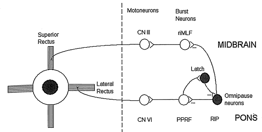
Figure 3-9. Schematic of brainstem network for saccade generation. Motoneurons innervating horizontally acting extraocular muscles receive saccadic commands from burst neurons in the paramedian pontine reticular formation (PPRF). Motoneurons innervating vertically acting motoneurons receive saccadic commands from burst neurons in the midbrain rostral interstitial nucleus of the medial longitudinal fasciculus (riMLF). Both sets of burst neurons are inhibited by omnipause neurons that lie in the pontine nucleus raphe interpositus (RIP). A saccade is initiated by a trigger signal that inhibits omnipause neurons; subsequently, hypothetical latch neurons, which receive input from burst neurons, inhibit omnipause neurons until the saccade is complete.
