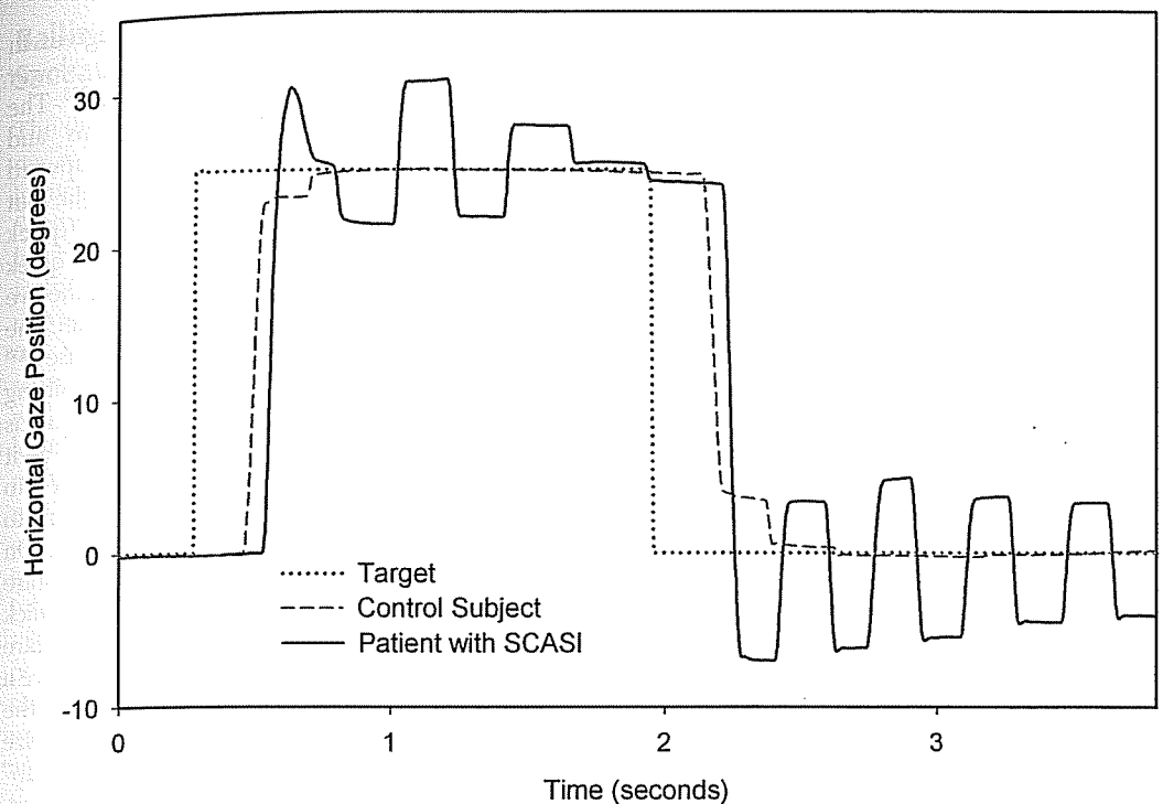
Figure 3–6. Examples of horizontal saccades made by a normal subject (gray, dashed line) and a patient with a spinocerebellar degeneration (solid line) in response to a 25-degree target jump (dotted line) from center position to right 25 degrees. After a reaction time, the normal subject makes an initial saccade that is hypometric, followed by a subsequent correction. A similar pattern occurs after the target returns to center. The patient shows hypermetria, overshooting the target when it jumps to the right, and especially when it jumps back to center, following which there are macrosaccadic oscillations about the point of fixation. 691 Positive values correspond to rightward movements.
