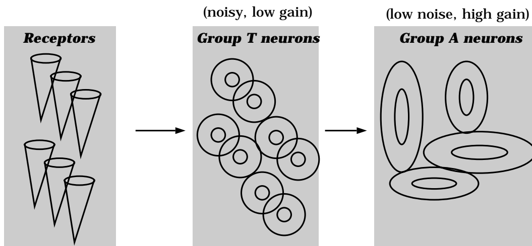
Figure 1.19: The neurons that limit detection and those that cause pattern adaptation may not be the same. For example, one group of neurons (Group T) may be noisy and have low contrast gain. Because of their noise properties, this group would limit detection threshold. Neurons in a second population (Group A) may integrate the responses of the first group of neurons and have high contrast gain. Because of their high gain, this group of neurons may fatigue easily and be the neural basis of pattern adaptation. If the neural units that limit these two types of behavioral responses are different, then the spatial receptive fields of neurons that are inferred from detection and pattern adaptation experiments may well be different.
