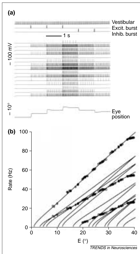
Fig. 4. Line attractor in a conductance-based memory model of oculomotor control.
