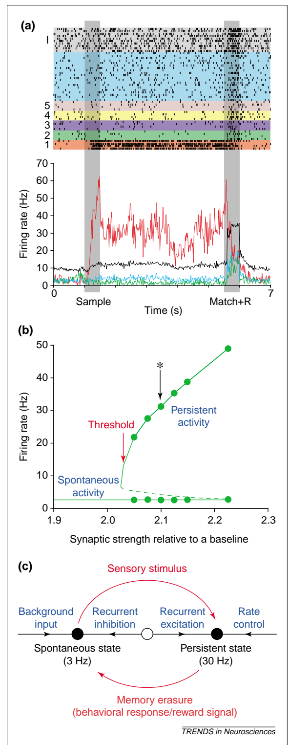
Fig. 2. Attractor paradigm for persistent activity. (a) Delayed match-to-sample simulation of an object working memory model 22 . Neural subpopulations (labeled 1 to 5) are selective to different stimuli. Average activity from each neural group is plotted below the rastergram. Inhibitory (I) cell population is shown in black. In the simulation, the shown stimulus triggers persistent activity in a pyramidal cell group (red) at about 30 Hz, but not in other pyramidal groups. Delay period activity is switched off by a transient excitatory input generating a brief surge of activity in all neurons. Adapted, with permission, from Ref. 65. (b) Dependence of network activity on the strength of recurrent synaptic connectivity. Solid lines: spontaneous state and persistent state; dashed line: unstable states. There is a critical threshold of synaptic strength, above which persistent activity appears abruptly as an all-or-none phenomenon. The example in (a) corresponds to the parameter indicated by the asterisk. (c) Illustration of the biophysics underlying an attractor dynamics. An attractor is a neural firing state that is stable to perturbations: when a small input perturbs the network to a lower or higher activity level, there is a 'restoring force' to bring the network back to the attractor state. In this case, the spontaneous state is stabilized from below by background inputs, and from above by feedback synaptic inhibition. The persistent activity state is stabilized from below by excitatory reverberation, and from above by various negative feedback 'rate control' mechanisms. A transient sensory stimulus can switch the network from the spontaneous state to the memory state, and a behavioral response or reward signal can turn the network off and erase the memory.
