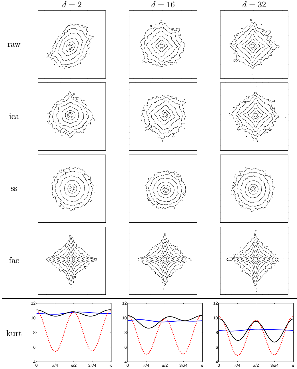
Figure 4: Contour plots of joint histograms of pairs of band-pass filter responses from an isotropic subband of the “boats” image with different spatial separations (given in units of pixels). See text for details.
