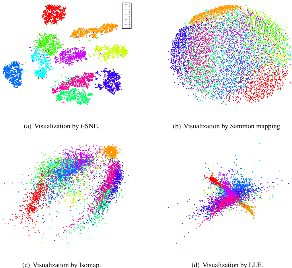
Figure 2: Visualizations of 6,000 handwritten digits from the MNIST dataset.
