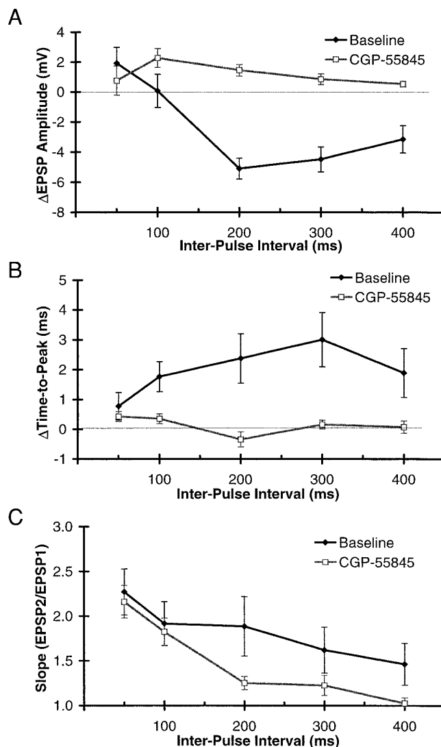
FIG. 5. Average effects of CGP-55845 on IPI functions for EPSP amplitude, TTP, and slope for hippocampal neurons. A: \Delta EPSP amplitude. In the control condition (black) facilitation of 2 mV was generally seen for the IPI of 50 ms, and depression was seen for the interval of >100 ms. CGP-55845 flattened the IPI function and abolished any depression of peak EPSP amplitude. B: \Delta TTPs were positive at all IPI, reflecting the increased TTP and broadening of the 2nd EPSP in relation to the 1st. CGP-55845 blocked the increases in TTP and again flattened the IPI function. C: EPSP slope was facilitated at all intervals but more so at the 50-ms IPI. CGP-55845 did not flatten the IPI function but did abolish most of the facilitation at the longer IPIs, which was largely due to increases in driving force produced by the slow IPSP.
