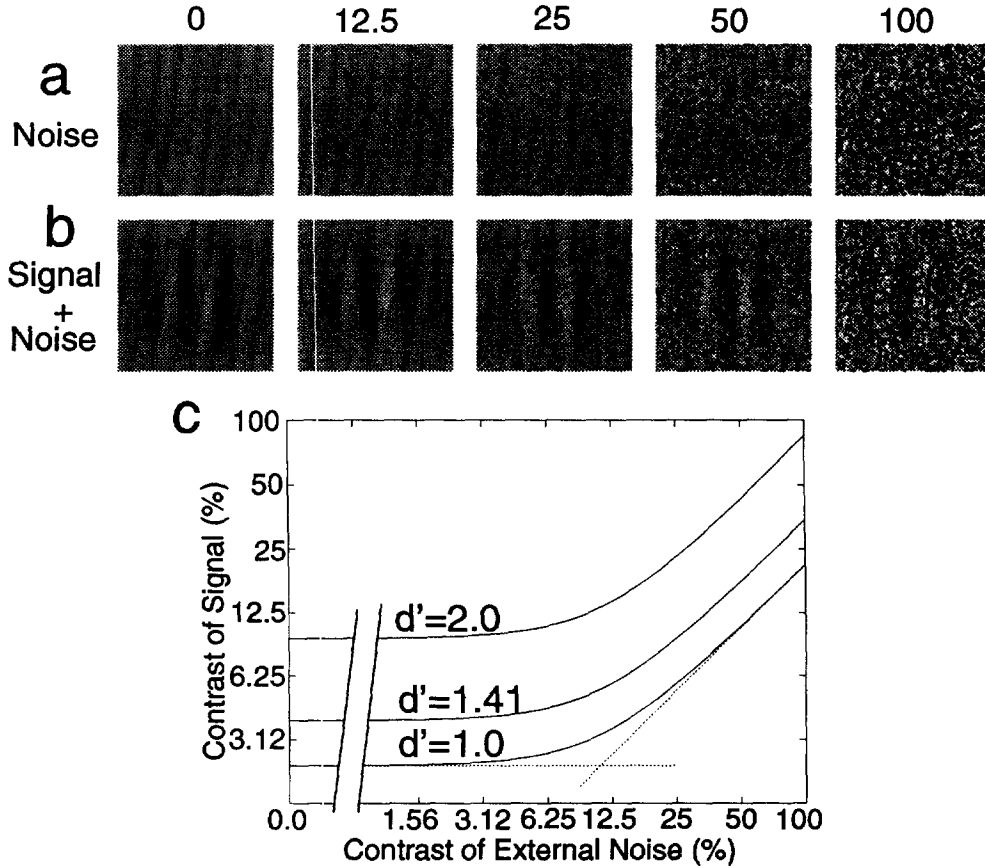
FIGURE 2. Contrast threshold of the noisy perceptual template model as a function of the contrast of the external noise for three different performance levels ( d' = 1, 1.41, 2.0 ). (a) External gaussian white noise. From left to right, the contrast of the noise increases from 0 to 100%. (b) Signal + external noise. Different amount of external gaussian noise (a) is linearly superimposed on a Gabor with constant contrast. The detectability of the Gabor deteriorates with the amplitude of the added external noise. (c) Contrast threshold of the noisy perceptual template model as a function of the external noise amplitude for three d' levels. For each d' level, the contrast threshold is a constant when the amplitude of the external noise is small; it increases with the amplitude of the external noise at high noise amplitudes. In that range, external noise dominates internal noise; performance is mostly determined by the amount of external noise.
