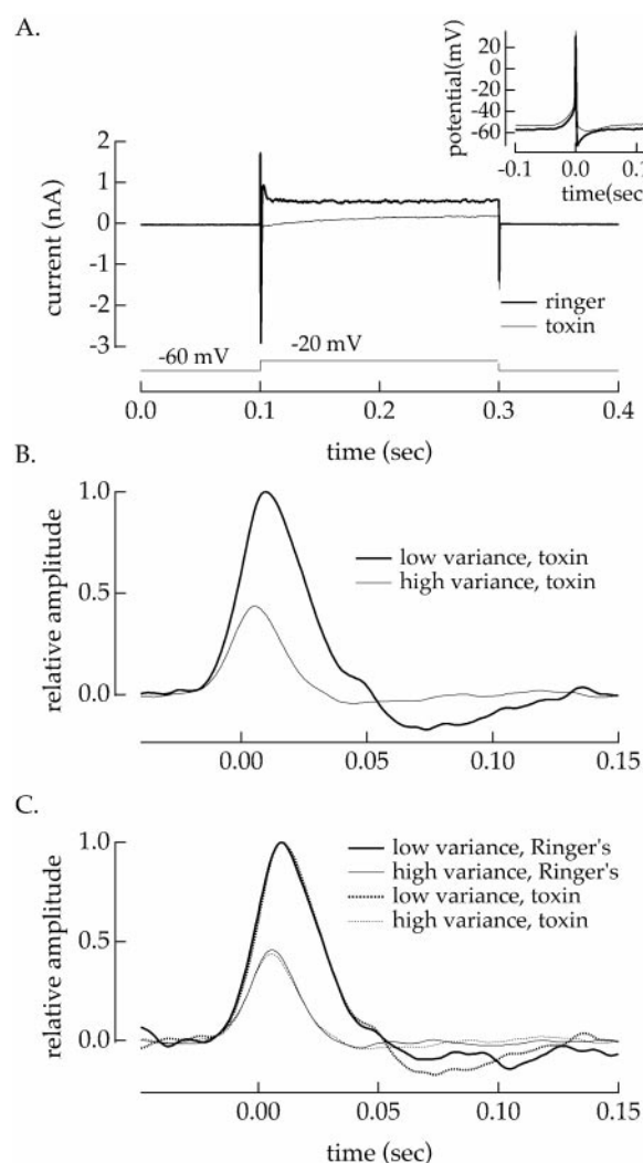
Figure 12. Adaptation to the current variance persisted with \text{Ca}^{2+} and \text{K}^+ currents suppressed. A , Suppression of \text{Ca}^{2+} and \text{K}^+ currents. The voltage of an isolated ganglion cell was stepped from -60 to -20 mV for 200 msec. The current responses in HEPES Ringer's solution ( thick line ) and in Ringer's solution with 200 \mu\text{M Ba}^{2+} , 400 \mu\text{M Cd}^{2+} , and 500 \text{ nM} apamin added ( thin line ) are shown. Suppression of \text{Ca}^{2+} and \text{K}^+ currents tripled the width at half-height of the average action potential and reduced the afterhyperpolarization ( inset ). B , Adaptation to changes in current variance without \text{Ca}^{2+} and \text{K}^+ currents. Gaussian noise (bandwidth 0–50 Hz) was injected into the cell under current clamp. Linear filters are shown for injected currents with variances of 16 \text{ pA}^2 ( thick trace ) and 144 \text{ pA}^2 ( thin traces ). C , Adaptation to changes in current variance was similar with and without \text{Ca}^{2+} and \text{K}^+ currents. Solid traces plot filters measured in HEPES Ringer's solution, and the dashed traces plot those measured with \text{Ca}^{2+} and \text{K}^+ currents suppressed. The filters in the absence of blockers were calculated with identical stimuli with and without toxins. Holding current was -10 to -16 \text{ pA} , chosen so the cell had similar mean firing rates in both conditions.
