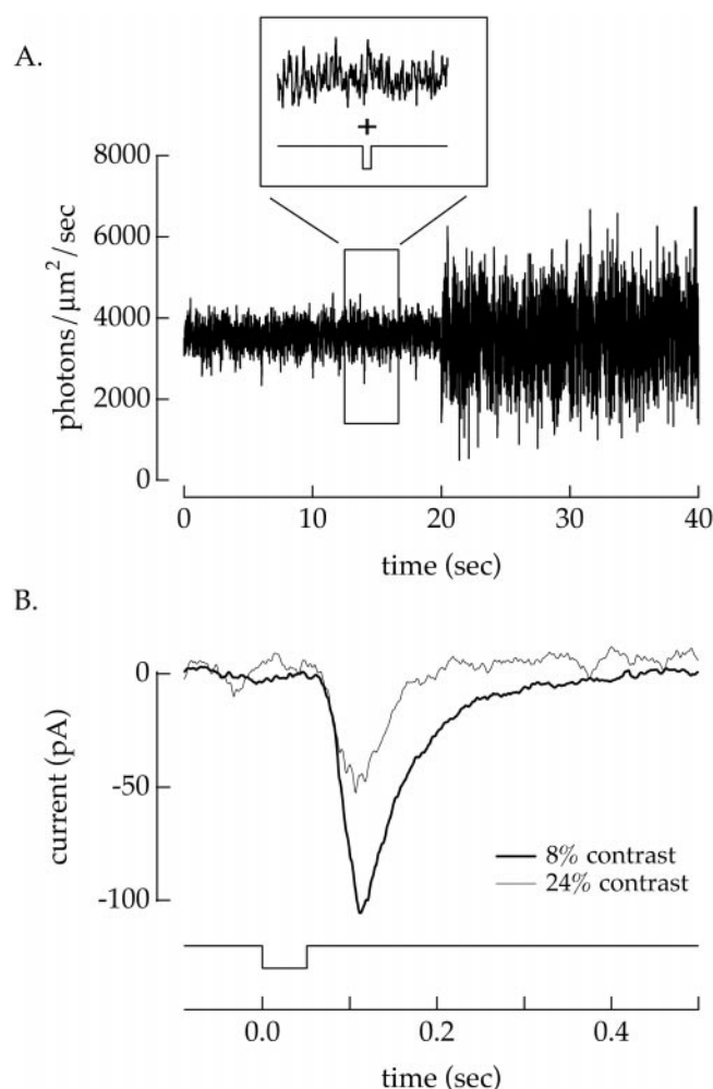
Figure 4. Temporal contrast affects the amplitude and kinetics of the input currents to a ganglion cell. A , Light stimulus used to test the effect of contrast on the flash response of the cell. The contrast was alternated between 8 and 24% every 20 sec. Every 2 sec a 20% L cone-isolating light decrement lasting 50 msec was superimposed on this alternating contrast signal ( inset ). B , Average current responses to the light decrement in the presence of 8% contrast and 24% contrast for an OFF ganglion cell. The averages of >20 responses all measured >10 sec after a change in contrast. Increasing the temporal contrast from 8 to 24% decreased the amplitude and sped the kinetics of the current response of the ganglion cell. Mean light intensity: 3560 photoisomerizations/sec per L cone; holding potential: -60 mV.
