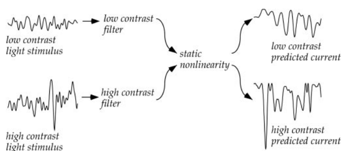
Figure 7. Effects of contrast in static nonlinearity model. The transformation of light input into the input current of a ganglion cell was described by a linear filter followed by a static nonlinearity. In 28 of 32 cells, the shape of the static nonlinearity was independent of the contrast of the light input, and hence the effect of contrast on the sensitivity was restricted to changes in the linear filter.
