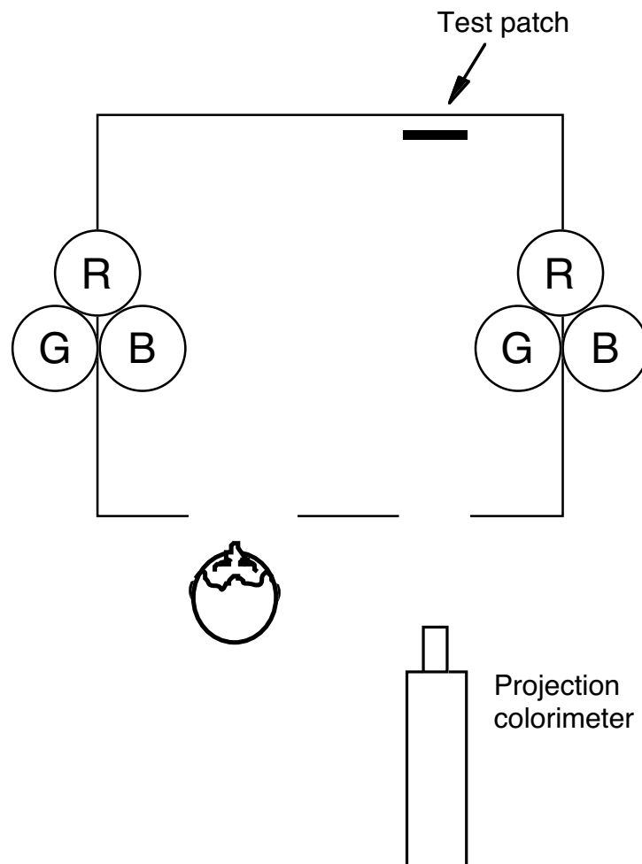
Figure 3. Schematic diagram of the experimental apparatus used in the experiments of Kraft and Brainard.
