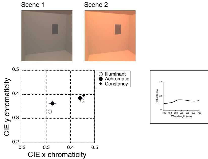
Figure 4. Basic data from achromatic adjustment experiment. The images at the top of the figure show the observer's view of two scenes, labeled 1 and 2. The test patch is visible in each image. The projection colorimeter was turned off at the time the images were acquired, so the images do not show the results of observers' achromatic adjustments. The chromaticity diagram shows the data from achromatic adjustments of the test patch made in the context of the two scenes. The open circles show the chromaticity of the illuminant for each scene. The illuminant for Scene 1 plots to the lower left of the illuminant for Scene 2. The closed circles show the chromaticity of the mean achromatic adjustments of four observers. Where visible, the error bars indicate \pm 1 standard error. The surface reflectance function plotted in the inset at the right of the figure shows the equivalent surface reflectance \tilde{S}(\lambda) computed from the data obtained in Scene 1. The closed diamond shows the color constant prediction for the achromatic adjustment in Scene 2, given the data obtained for Scene 1. See explanation in the text.
