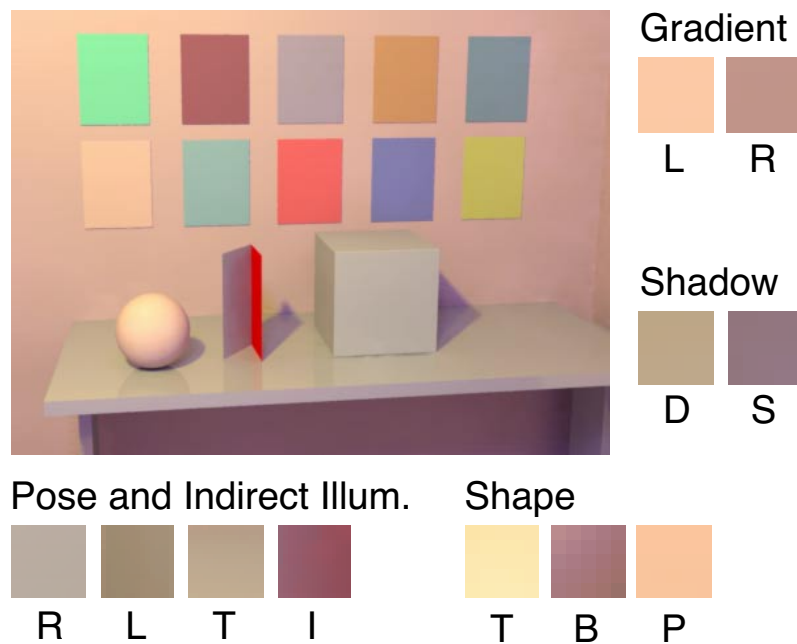
Figure 2. Image formation. Each set of square patches around the side of the image illustrate variation in the light reflected to the eye when surface reflectance is held fixed. Gradient: The two patches shown were extracted from the upper left (L) and lower right (R; above table) of the back wall of the scene. Shadow. The two patches were extracted from the tabletop in direct illumination (D) and shadow (S). Shape: The three patches shown were extracted from two regions of the sphere (T and B; center top and right bottom respectively) and from the colored panel directly above the sphere (P; the panel is the leftmost of the four in the bottom row). Both the sphere and panel have the same simulated surface reflectance function. Pose and Indirect Illum. The four patches were extracted from the three visible sides of the cube (R, L, and T; right, left and top visible sides respectively) and from the left side of the folded paper located between the cube and sphere (I). The simulated surface reflectance of all sides of the cube and of the left side of the folded paper are identical. The image was rendered from a synthetic scene description using the Radiance computer graphics package (Larson & Shakespeare, 1998). There were two sources of illumination in the simulated scene: a diffuse illumination that would appear bluish if viewed in isolation and a directional illumination (from upper left) that would appear yellowish if viewed in isolation. All of the effects illustrated by this rendering are easily observed in natural scenes.
