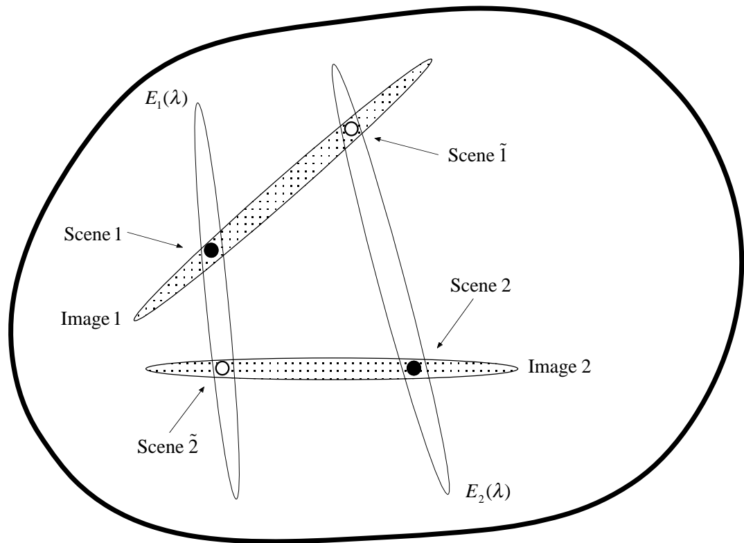
Figure 5. Schematic illustration of the ambiguity inherent in color constancy. The figure shows, schematically, the set of all scenes. Each point in the schematic represents a possible scene. Scenes 1 and 2 from the experiment described above are indicated by closed circles. Each hatched ellipse encloses a subset of scenes that all produce the same image. The scenes represented by open circles, Scenes \tilde{1} and \tilde{2} , produce the same images as Scenes 1 and 2 respectively. The open ellipses each enclose a subset of scenes that share the same illuminant.
