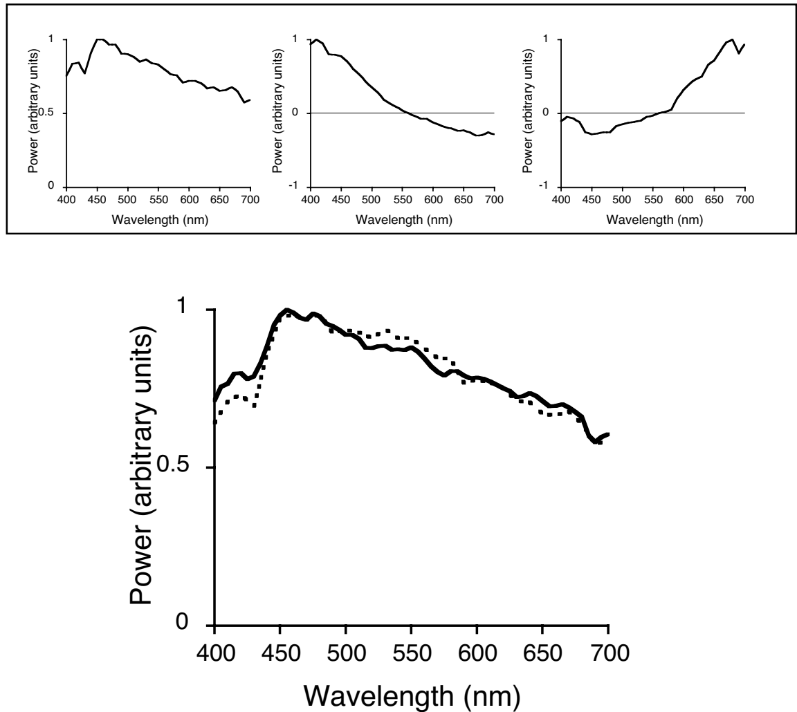
Figure 7. Linear model for natural daylights. Top) Three basis functions for the CIE linear model for daylights (CIE, 1986). Bottom) Linear model approximation to a measured daylight. Solid line, measurement. Dotted line, reconstruction. The measured daylight was obtained from a database of measurements made available by J. Parkkinen and P. Silfsten on the world-wide web at URL http://cs.joensuu.fi/~spectral/databases/download/daylight.htm
