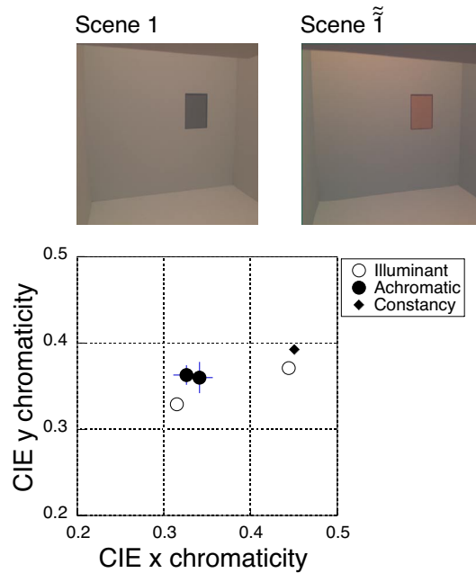
Figure 6. Achromatic data when both illuminant and scene surfaces are varied. The images at the top of the figure show the observer's view of two scenes, labeled 1 and \tilde{1} . The relation between these scenes is described in the text. The test patch is visible in each image. The projection colorimeter was turned off at the time the images were acquired, so the images do not show the results of observers' achromatic adjustments. The chromaticity diagram shows the data from achromatic adjustments of the test patch made in the context of the two scenes. Same format as Figure 4. The equivalent surface reflectance \tilde{S}(\lambda) computed from the data obtained in Scene 1 is shown in Figure 4.
