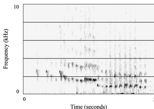
Fig. 7. Spectrogram of a tamarin alarm call.
