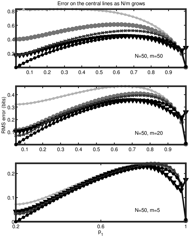
Figure 6: “Central line” error curves for three different values of N/m (notation as in Figure 5). Note that the worst-case error of the new estimator is less than that of the three most common \hat{H} for all observed (N, m) pairs and that the error curves for the four estimators converge to the CLT curve as N/m \rightarrow \infty .
