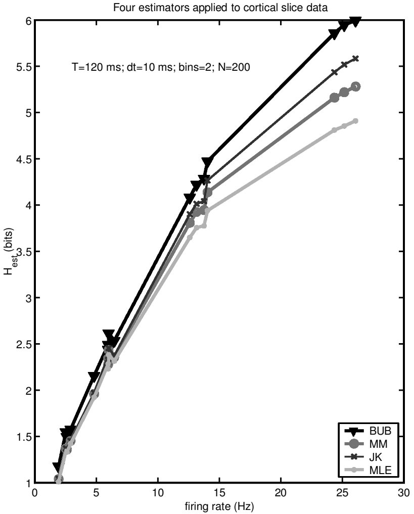
Figure 9: Estimated entropy of spike trains from a single cell recorded in vitro. The cell was driven with a white noise current. Each point corresponds to a single experiment, with N = 200 i.i.d. trials. The standard deviation of the input noise was varied from experiment to experiment. Spike trains were 120 ms long, discretized into 10 ms bins of 0 or 1 spike each; m = 2^{12} .
