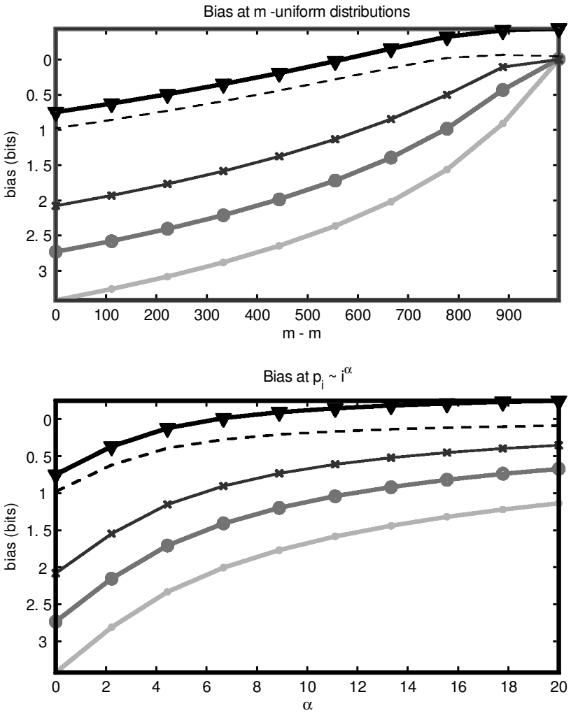
Figure 7: Exact bias on two additional families of distributions. The notation is as in Figure 5; the dashed line corresponds to \hat{H}_{BUB} with \lambda_0 set to reduce the bias at the zero-entropy point. (Top) Flat distributions on m' bins, 1 \leq m' \leq m . (Bottom) p_i \sim i^{-\alpha} . N = 100 and m = 1000 in each panel.
