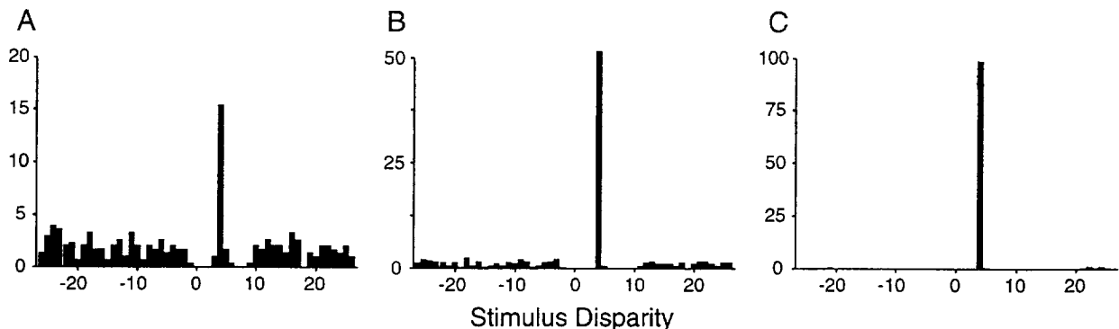
FIGURE 12. Simulations like that in Fig. 11 were run 300\times with statistically independent white noise stimuli. Position-shifted energy neurons were tuned to a disparity of 4 pixels. Each histogram plots the percentage of times that the peak response occurred at each disparity. (A) Responses of a single energy neuron show a wide range of false peaks, with only 18% of the peaks falling within 1 pixel of the correct disparity. (B) Pooling over orientation and space yields a sharper concentration of peaks, but still only 52% of the peaks within 1 pixel of the correct disparity. (C) After pooling over scale, orientation, and space, 99% of the peaks lie at the correct disparity.
