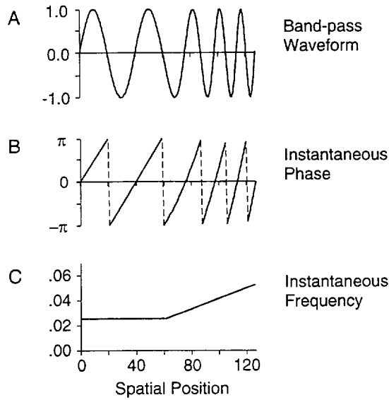
FIGURE 7. (A) Quasi-sinusoidal signal, the frequency of which varies with spatial location; the frequency is constant from locations 0 to 60, after which it increases linearly. (B) The corresponding phase signal. (C) Instantaneous frequency, which is the derivative of the phase signal. When stimulus frequency is constant, the phase signal increases linearly and the instantaneous frequency is constant. When frequency increases, so does the slope of the phase signal, which is the instantaneous frequency.
