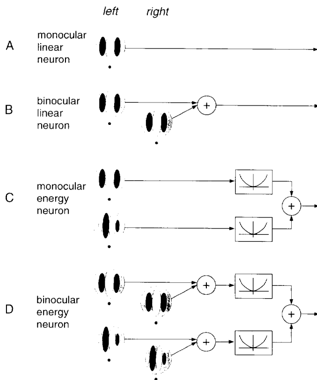
FIGURE 1. Receptive fields of model neurons. (A) A monocular, orientation-selective linear neuron. Its response depends on a weighted sum of the stimulus intensities within its receptive field. Shaded ellipses correspond to inhibitory subregions of the weighting function and the unshaded ellipse corresponds to an excitatory subregion. (B) A binocular linear neuron's response depends on a weighted sum of the stimulus intensities presented to both eyes. The reference points (black dots) below the weighting functions indicate that the two weighting functions are in exact binocular correspondence. (C) A monocular energy neuron sums the squared responses of two monocular linear neurons. The weighting functions of the two linear neurons are identical except for a 90 deg phase shift. (D) A binocular energy neuron sums the squared responses of two binocular linear neurons. All four linear weighting functions are centered in exact (monocular and binocular) retinal correspondence.
