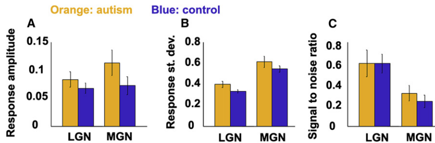
Figure 6. Subcortical Responses
